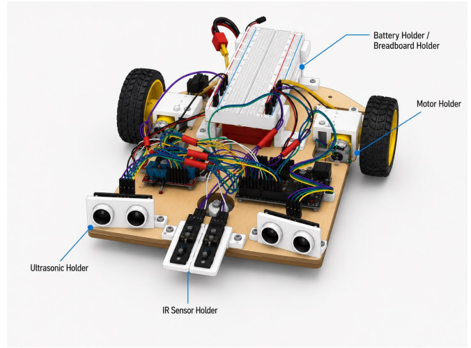
Fig. 7. Holder Placement on the Robot Chassis
